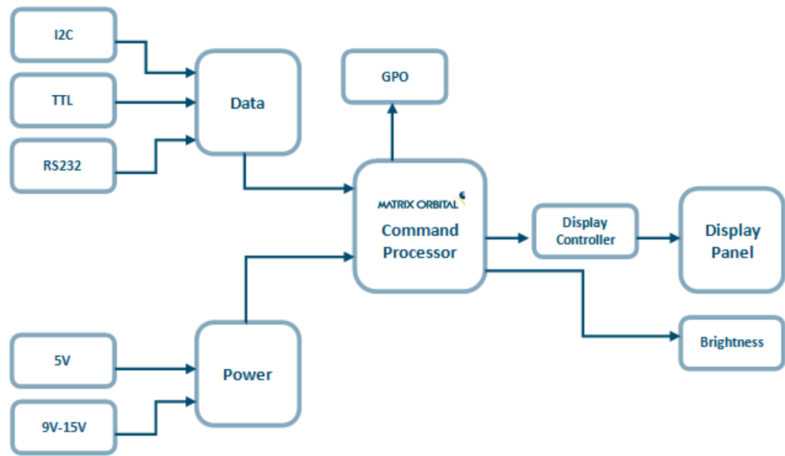
Figure 10: Functional Diagram
